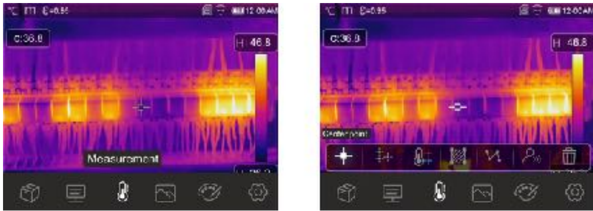
Fig. 34: Measurement Menu
